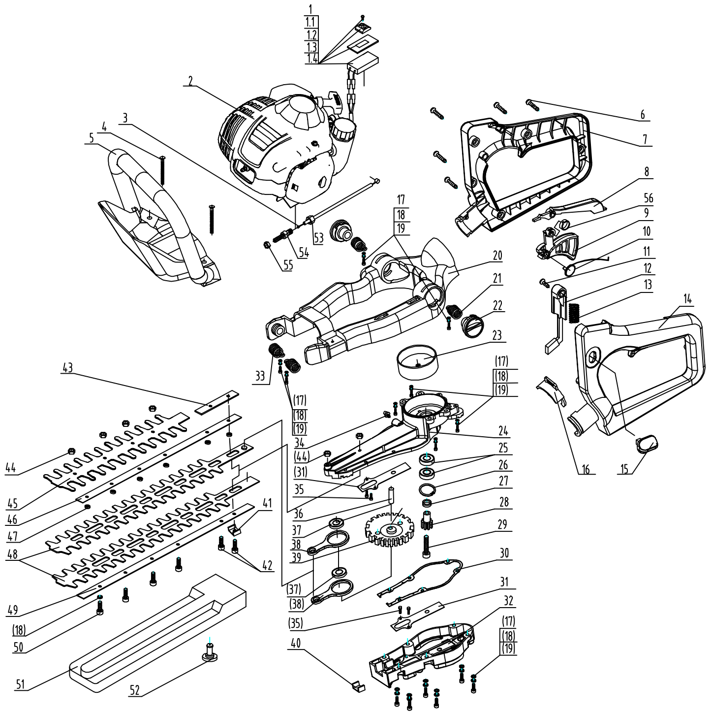
The parts list for hedge Trimmer explode chart of MQE-3SPK-560 (product coding A450000)
