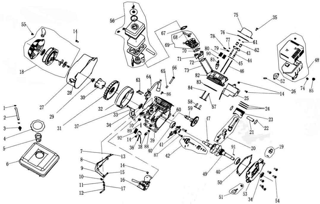
SR168F/P、SR168F/P-2、SR170F/P爆炸图(explode view list)
