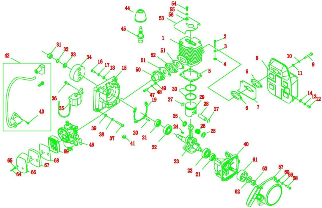
FIG. 1: 1E40F-3Z GASOLINE ENGINE
