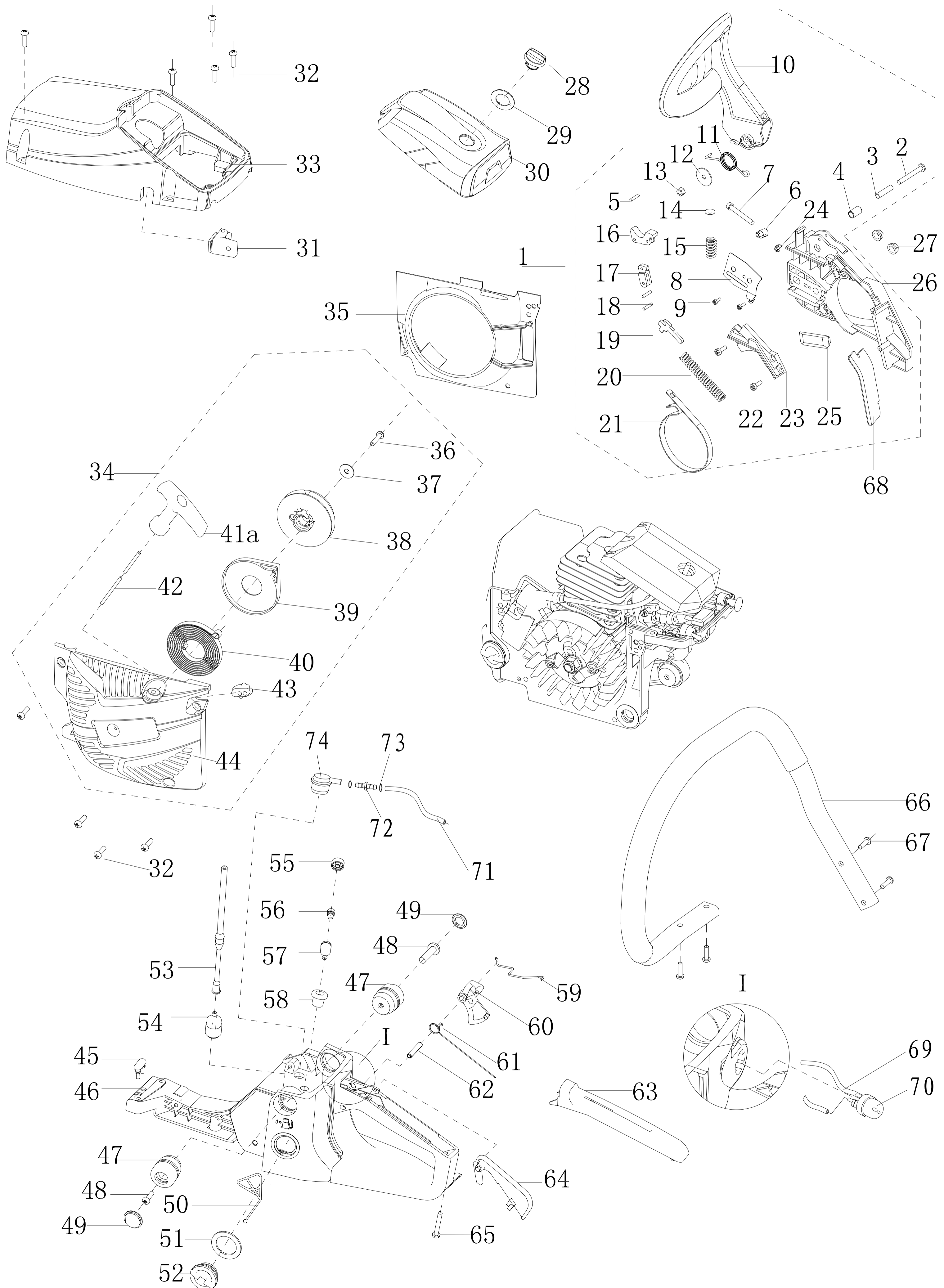
BASE UNIT
